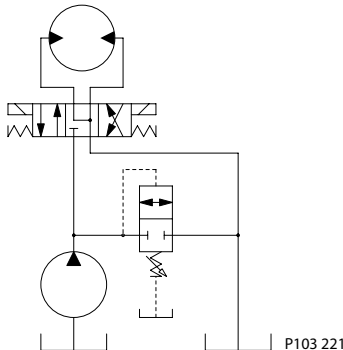
Sequence valve as relief
