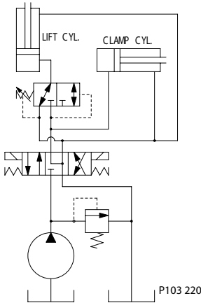
Clamp & lift circuit
